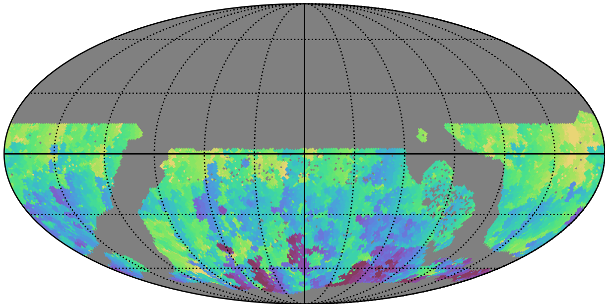
ddf_acor_sf10_lsf20_lsr50_v3.4_10yrs WFD u band: Min HA
