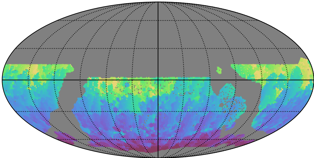
ddf_acor_sf10_lsf20_lsr50_v3.4_10yrs WFD g band: Min HA
