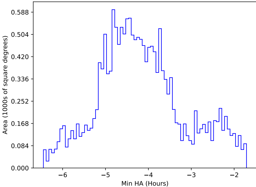
ddf_acor_sf10_lsf20_lsr50_v3.4_10yrs WFD g band: Min HA
