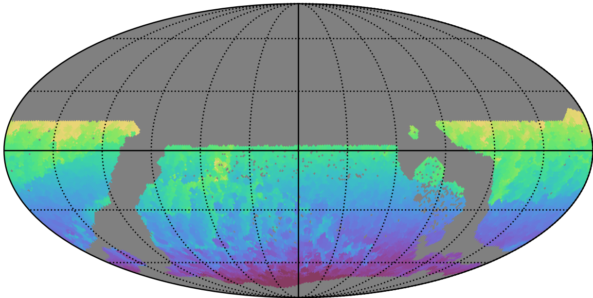
ddf_acor_sf10_lsf20_lsr50_v3.4_10yrs WFD all bands: Min HA
