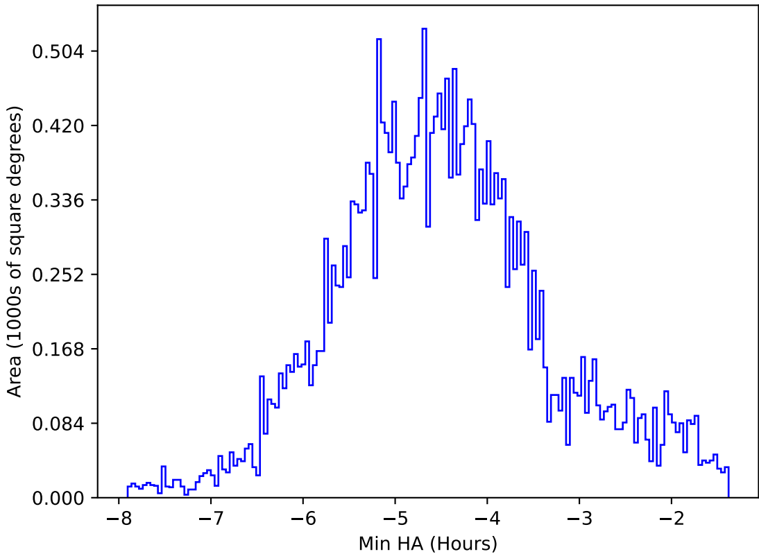
ddf_acor_sf10_lsf20_lsr50_v3.4_10yrs All sky all bands: Min HA
