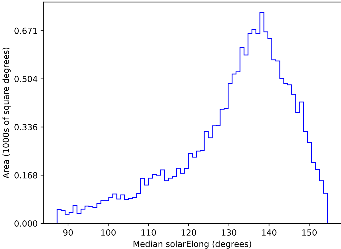
ddf_acor_sf10_lsf20_lsr50_v3.4_10yrs WFD u band: Median solarElong
