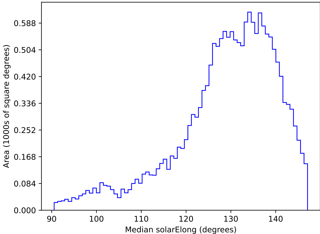
ddf_acor_sf10_lsf20_lsr50_v3.4_10yrs WFD i band: Median solarElong
