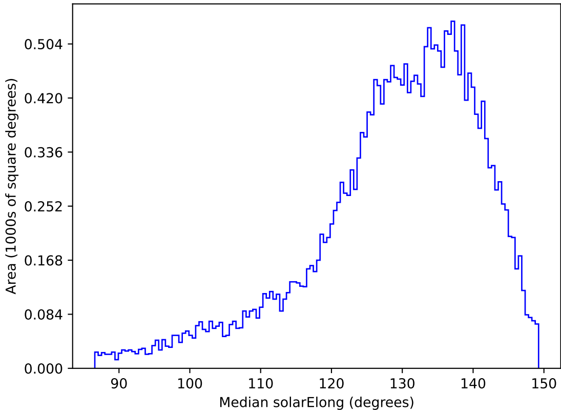
ddf_acor_sf10_lsf20_lsr50_v3.4_10yrs All sky i band: Median solarElong
