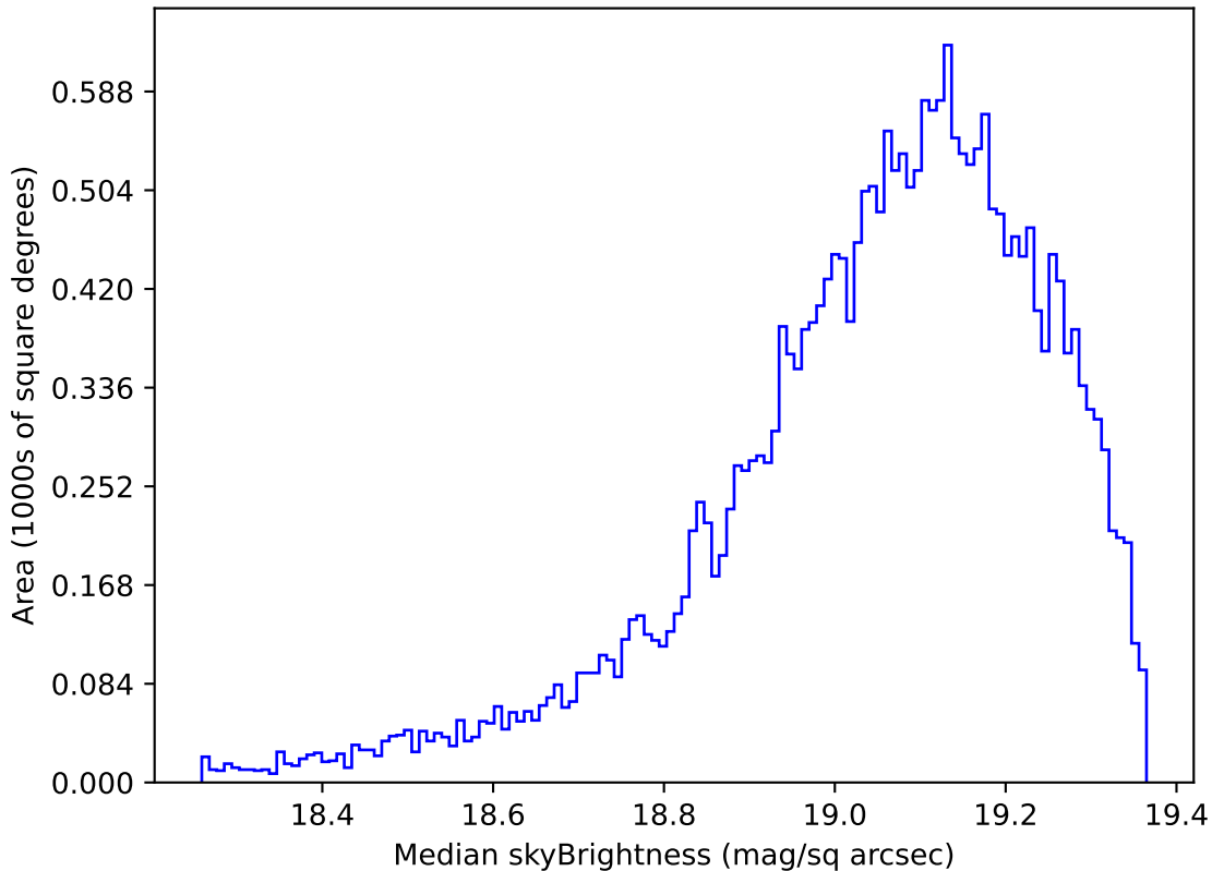
ddf_acor_sf10_lsf20_lsr50_v3.4_10yrs Yr 1 z band: Median skyBrightness
