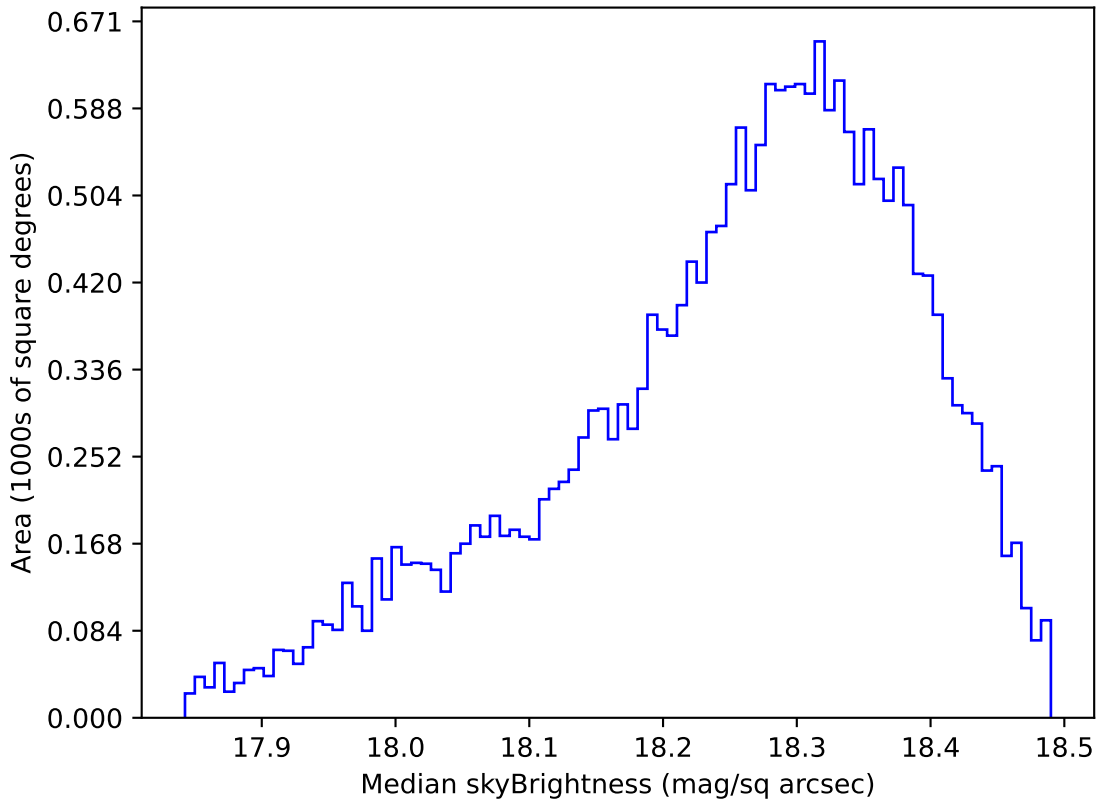
ddf_acor_sf10_lsf20_lsr50_v3.4_10yrs Yr 1 y band: Median skyBrightness
