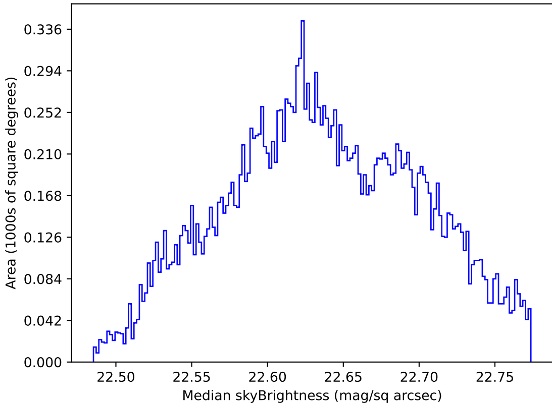
ddf_acor_sf10_lsf20_lsr50_v3.4_10yrs Yr 1 u band: Median skyBrightness
