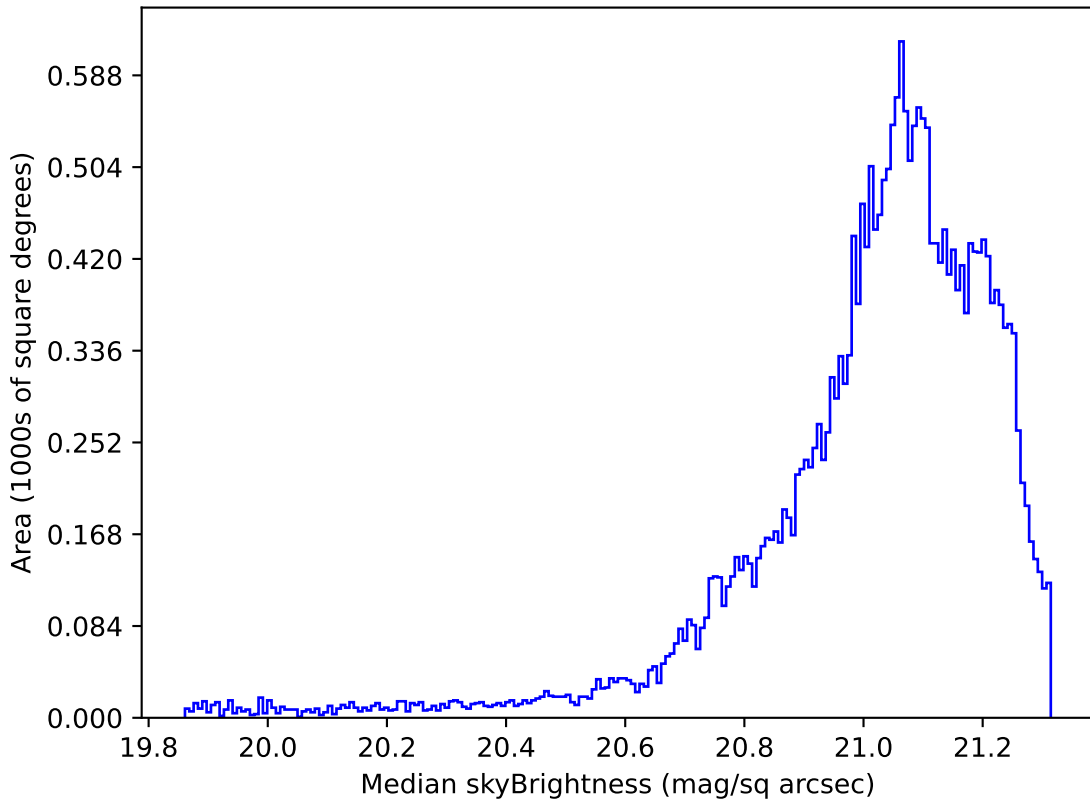
ddf_acor_sf10_lsf20_lsr50_v3.4_10yrs Yr 1 r band: Median skyBrightness
