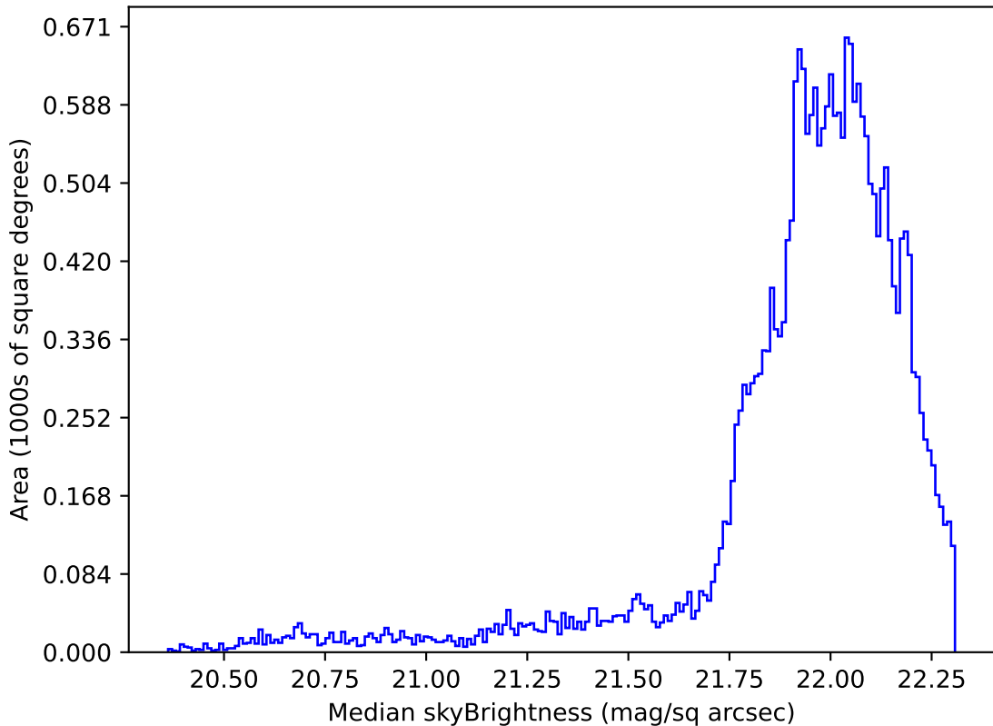
ddf_acor_sf10_lsf20_lsr50_v3.4_10yrs Yr 1 g band: Median skyBrightness
