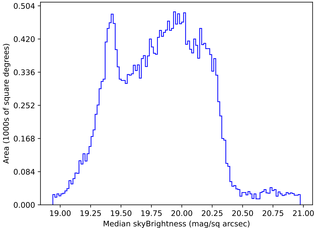
ddf_acor_sf10_lsf20_lsr50_v3.4_10yrs Yr 1 all bands: Median skyBrightness
