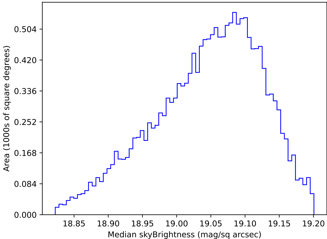
ddf_acor_sf10_lsf20_lsr50_v3.4_10yrs WFD z band: Median skyBrightness
