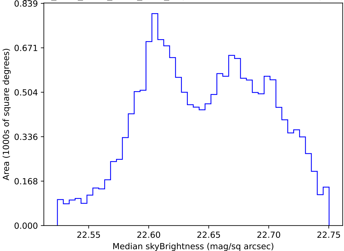
ddf_acor_sf10_lsf20_lsr50_v3.4_10yrs WFD u band: Median skyBrightness
