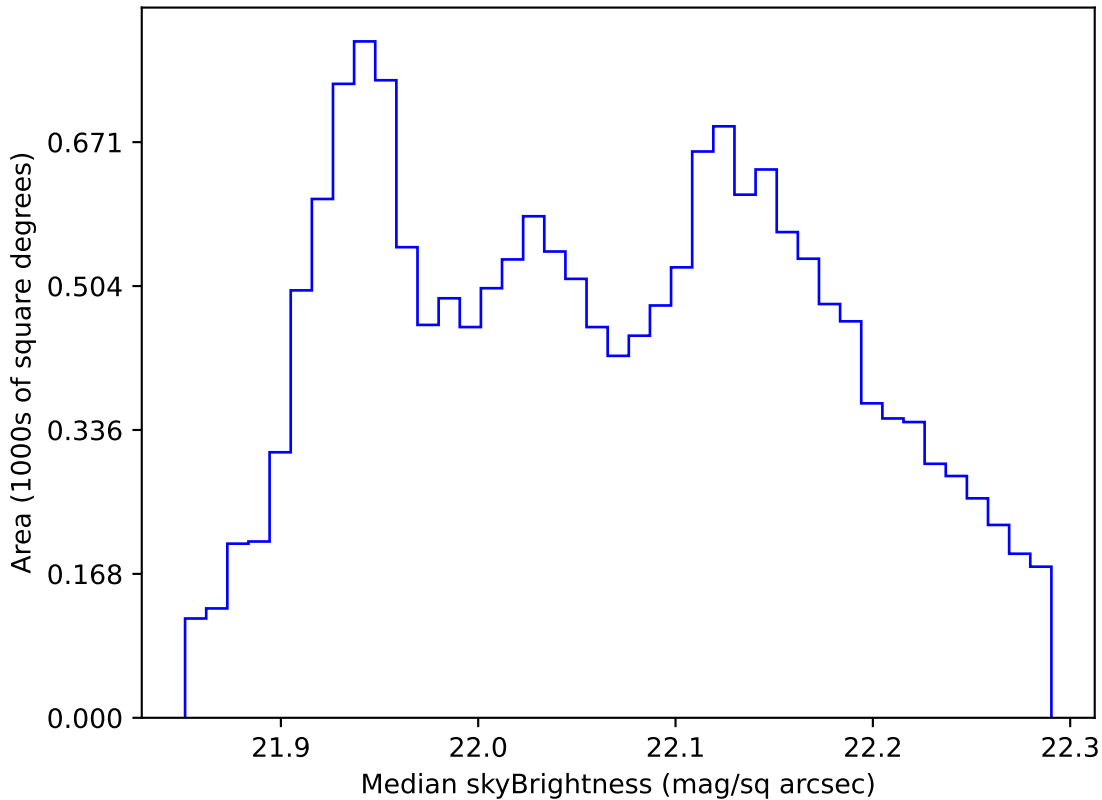
ddf_acor_sf10_lsf20_lsr50_v3.4_10yrs WFD g band: Median skyBrightness
