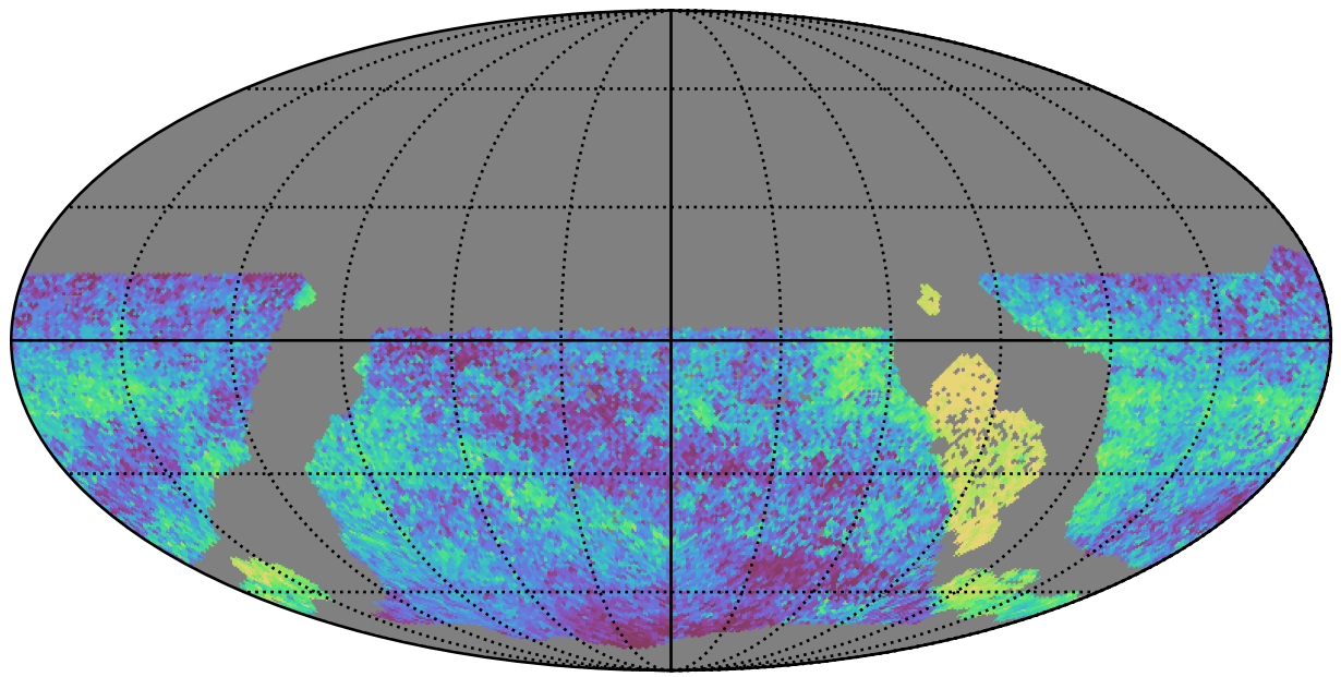
ddf_acor_sf10_lsf20_lsr50_v3.4_10yrs WFD all bands: Median skyBrightness
