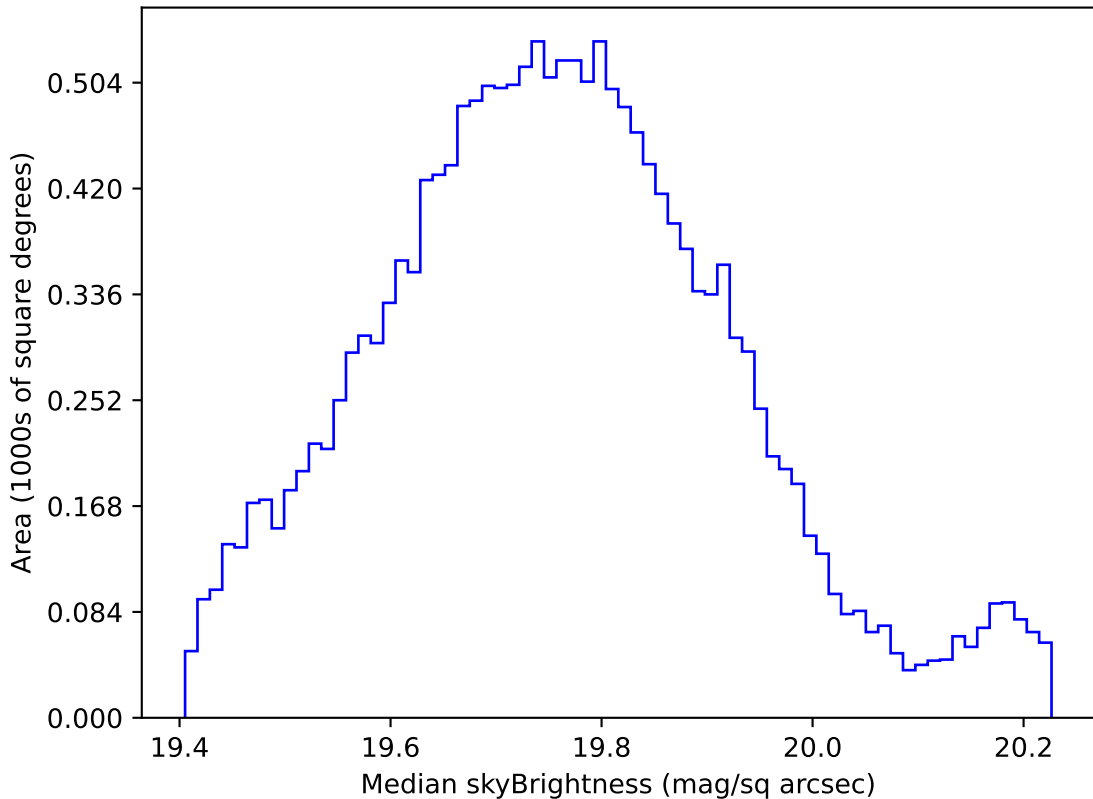
ddf_acor_sf10_lsf20_lsr50_v3.4_10yrs WFD all bands: Median skyBrightness
