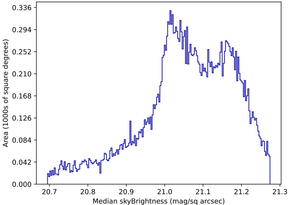
ddf_acor_sf10_lsf20_lsr50_v3.4_10yrs All sky r band: Median skyBrightness
