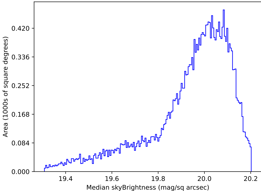
ddf_acor_sf10_lsf20_lsr50_v3.4_10yrs All sky i band: Median skyBrightness
