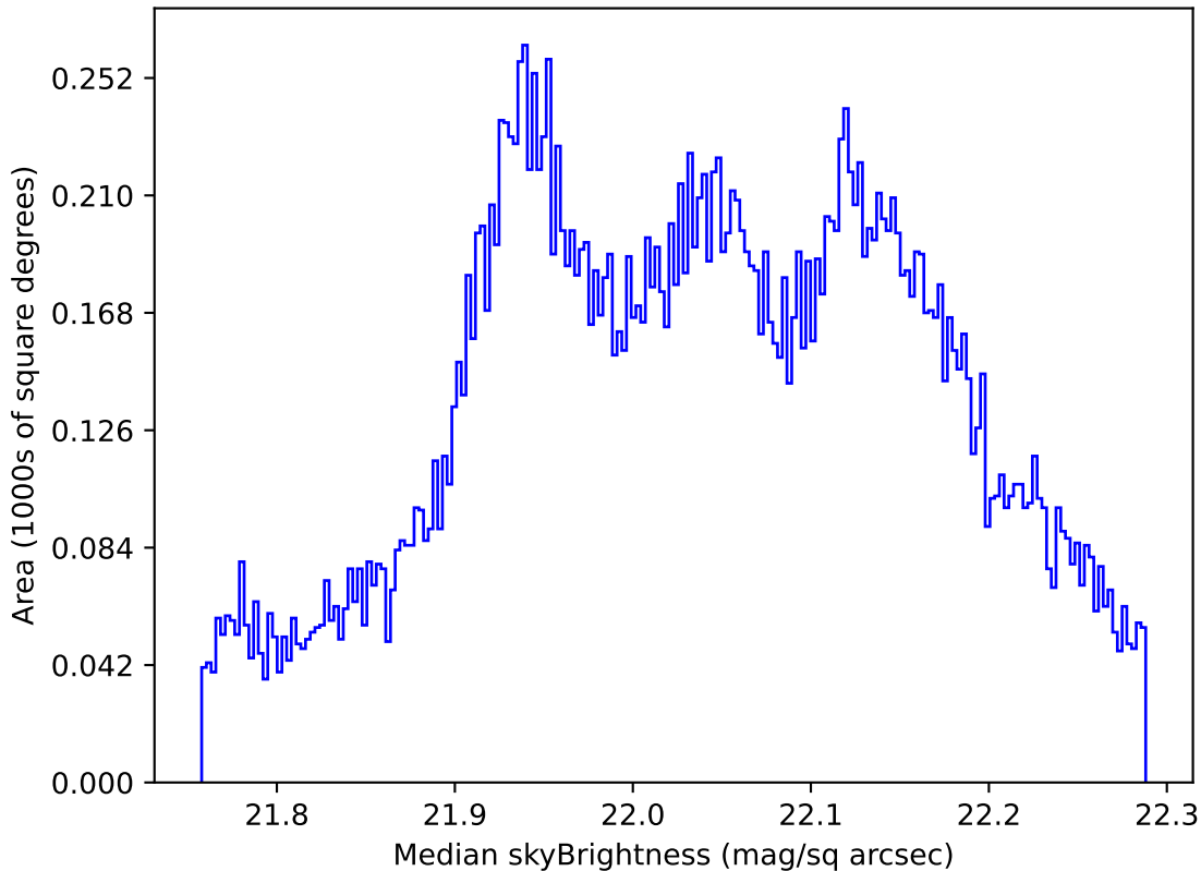
ddf_acor_sf10_lsf20_lsr50_v3.4_10yrs All sky g band: Median skyBrightness
