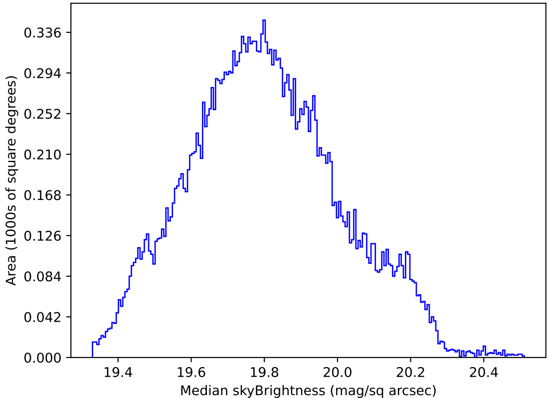
ddf_acor_sf10_lsf20_lsr50_v3.4_10yrs All sky all bands: Median skyBrightness
