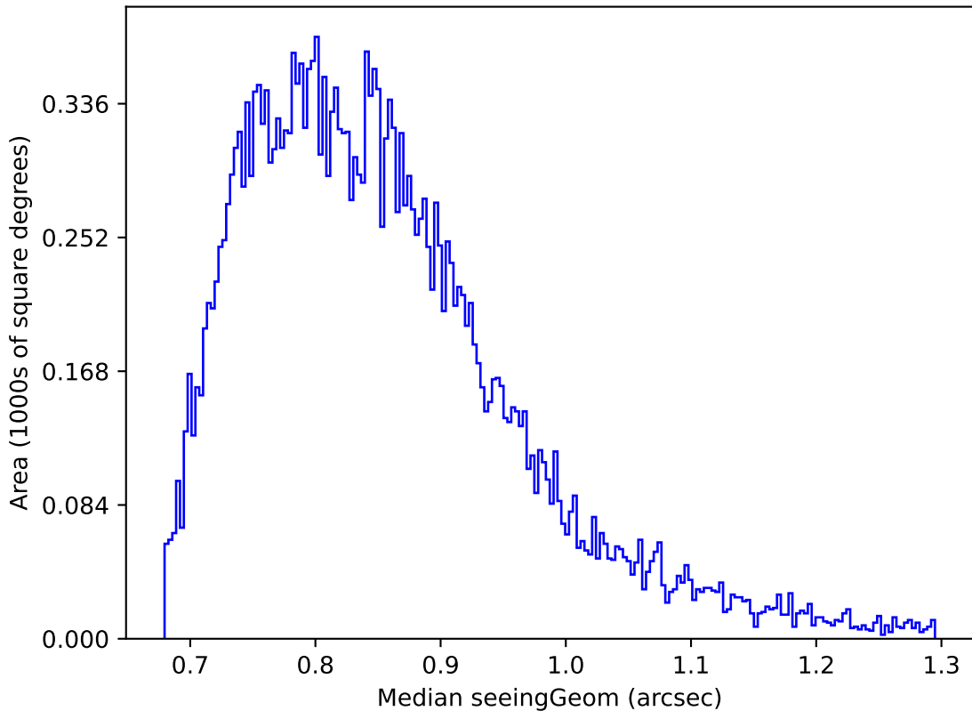
ddf_acor_sf10_lsf20_lsr50_v3.4_10yrs Yr 1 z band: Median seeingGeom
