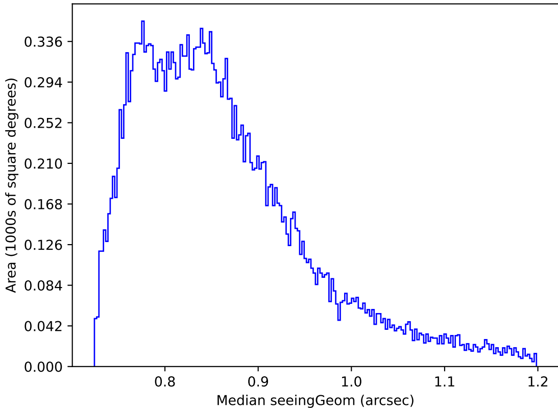
ddf_acor_sf10_lsf20_lsr50_v3.4_10yrs Yr 1 all bands: Median seeingGeom
