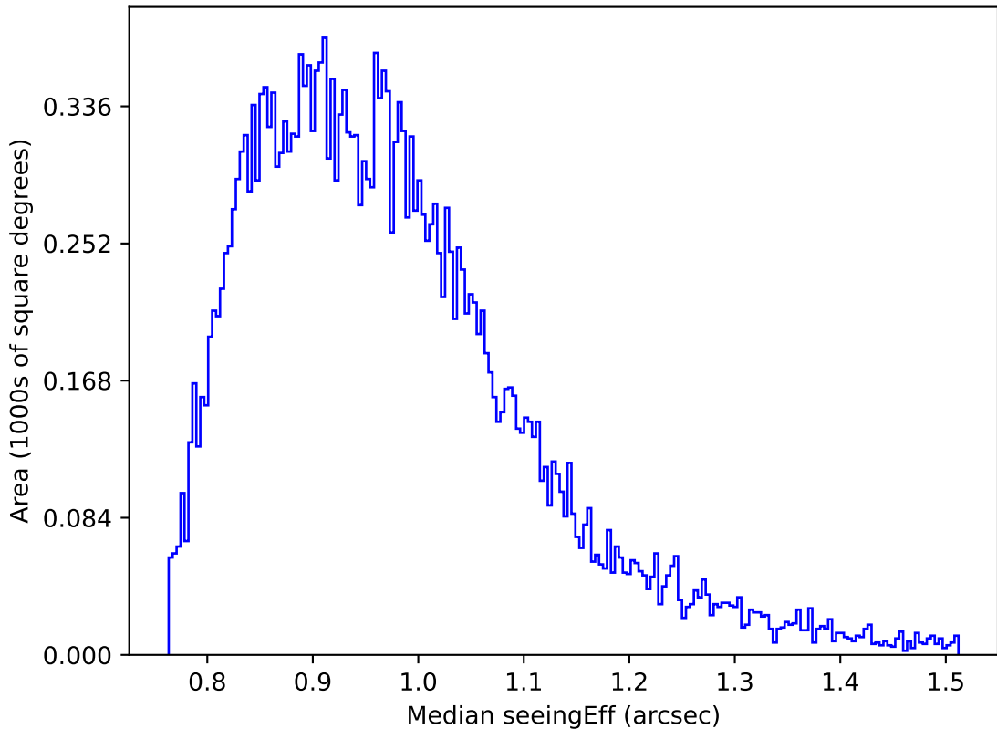
ddf_acor_sf10_lsf20_lsr50_v3.4_10yrs Yr 1 z band: Median seeingEff
