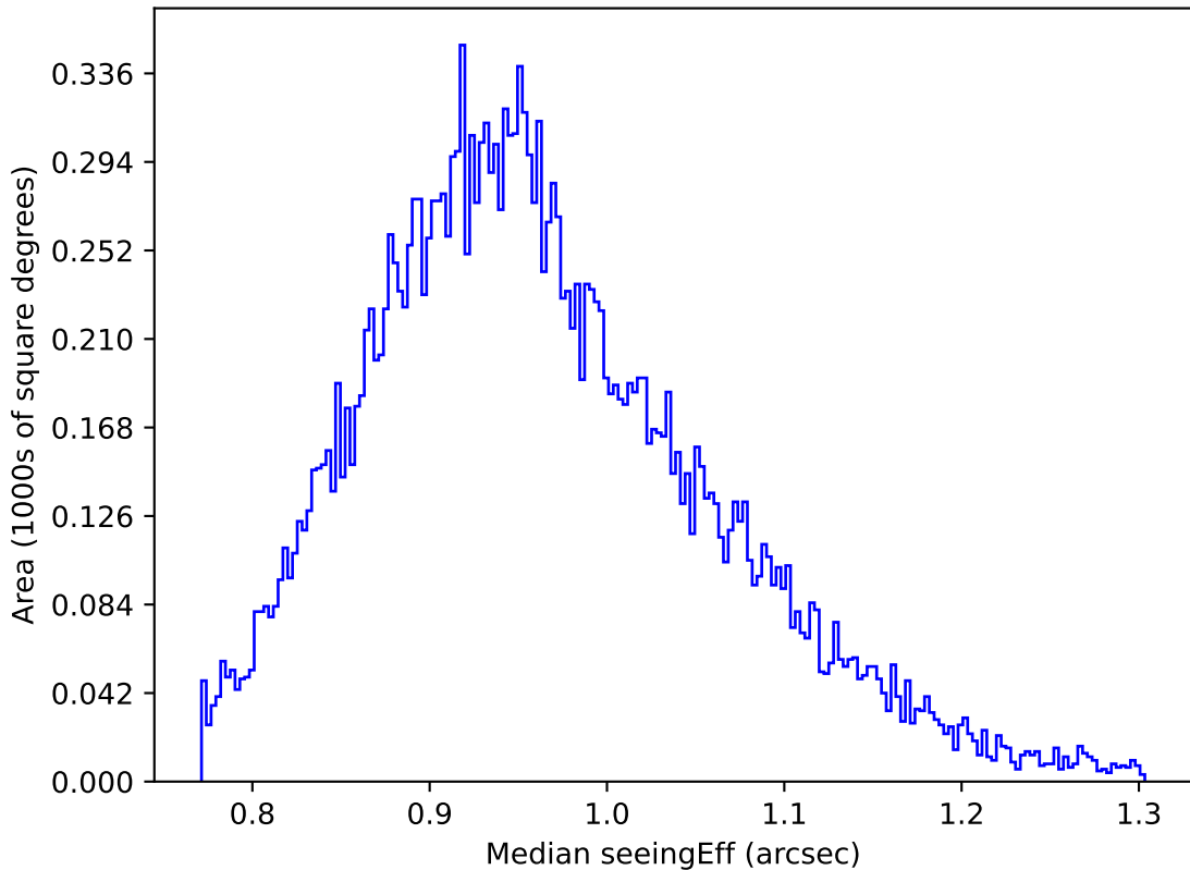
ddf_acor_sf10_lsf20_lsr50_v3.4_10yrs Yr 1 y band: Median seeingEff
