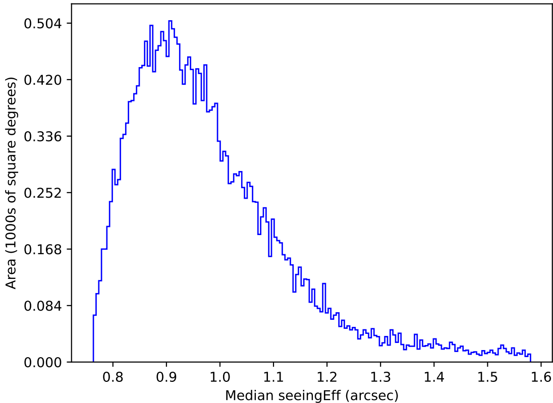
ddf_acor_sf10_lsf20_lsr50_v3.4_10yrs Yr 1 r band: Median seeingEff
