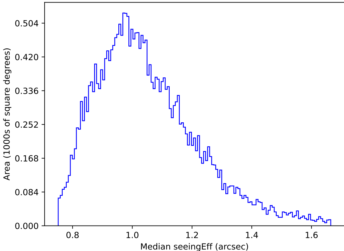
ddf_acor_sf10_lsf20_lsr50_v3.4_10yrs Yr 1 g band: Median seeingEff
