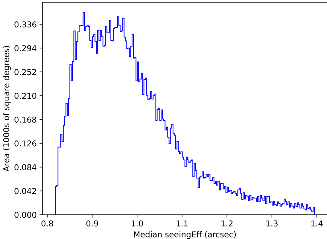
ddf_acor_sf10_lsf20_lsr50_v3.4_10yrs Yr 1 all bands: Median seeingEff
