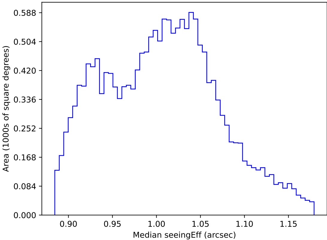
ddf_acor_sf10_lsf20_lsr50_v3.4_10yrs WFD y band: Median seeingEff
