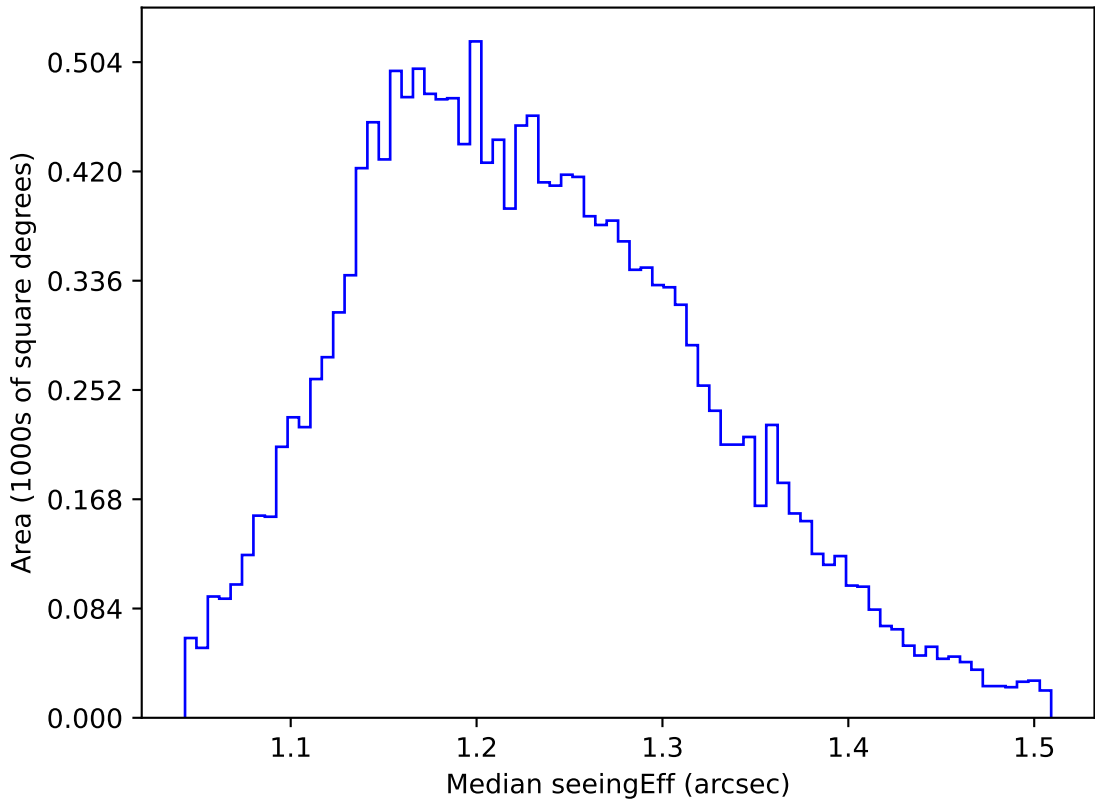
ddf_acor_sf10_lsf20_lsr50_v3.4_10yrs WFD u band: Median seeingEff
