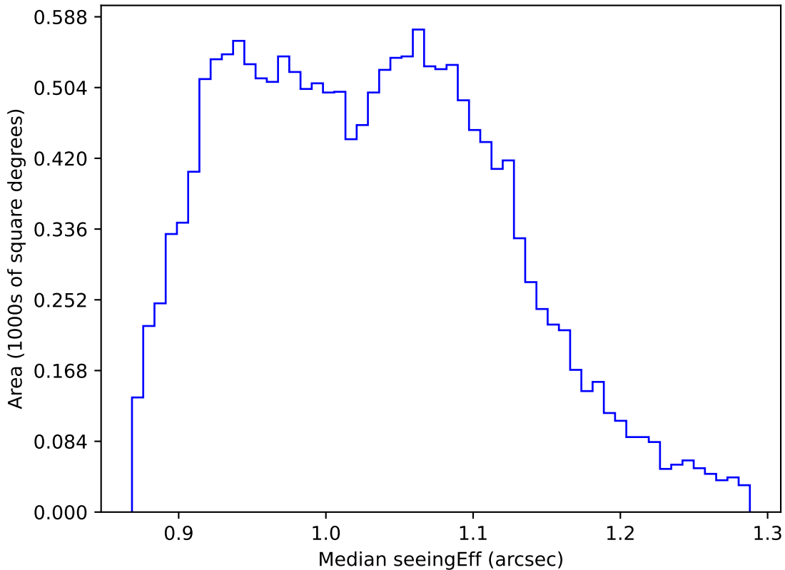
ddf_acor_sf10_lsf20_lsr50_v3.4_10yrs WFD r band: Median seeingEff
