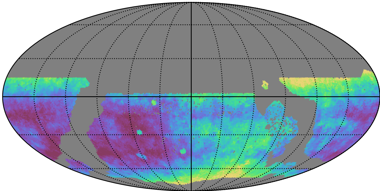
ddf_acor_sf10_lsf20_lsr50_v3.4_10yrs WFD i band: Median seeingEff
