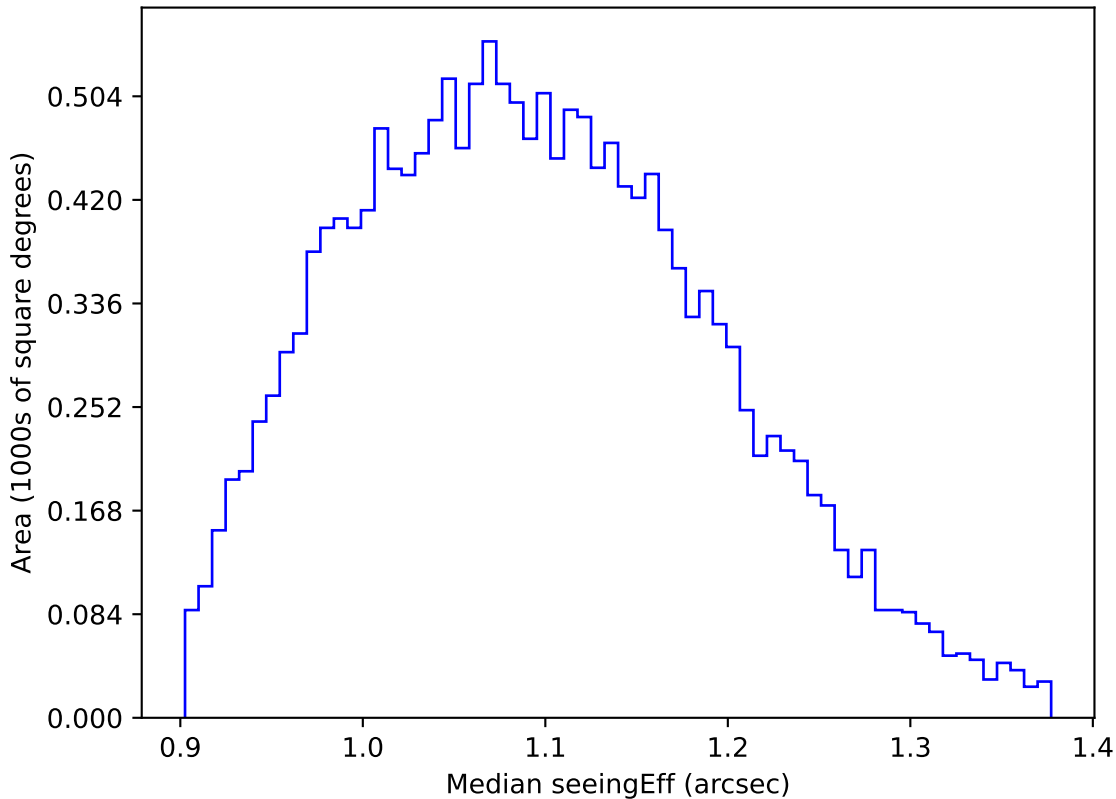
ddf_acor_sf10_lsf20_lsr50_v3.4_10yrs WFD g band: Median seeingEff
