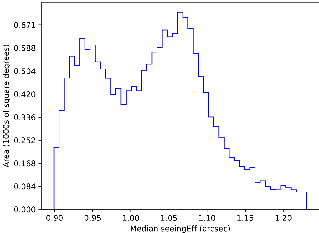
ddf_acor_sf10_lsf20_lsr50_v3.4_10yrs WFD all bands: Median seeingEff
