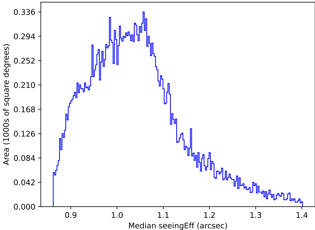
ddf_acor_sf10_lsf20_lsr50_v3.4_10yrs All sky z band: Median seeingEff
