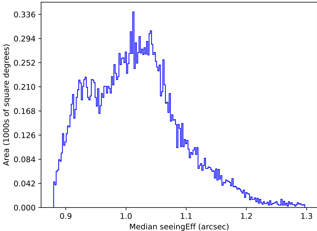
ddf_acor_sf10_lsf20_lsr50_v3.4_10yrs All sky y band: Median seeingEff
