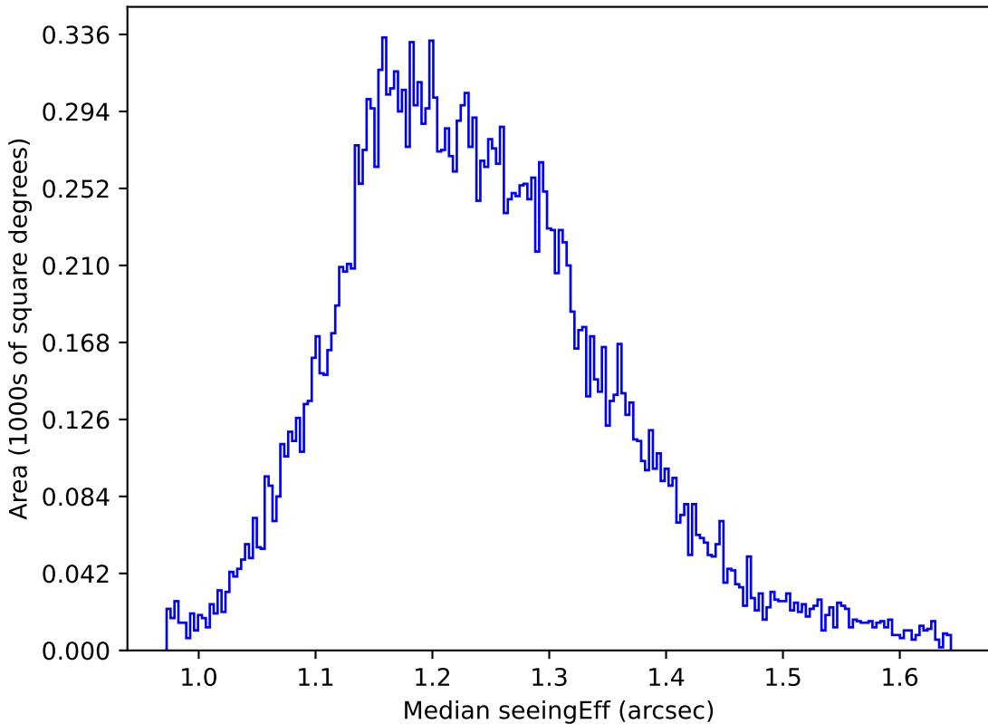
ddf_acor_sf10_lsf20_lsr50_v3.4_10yrs All sky u band: Median seeingEff
