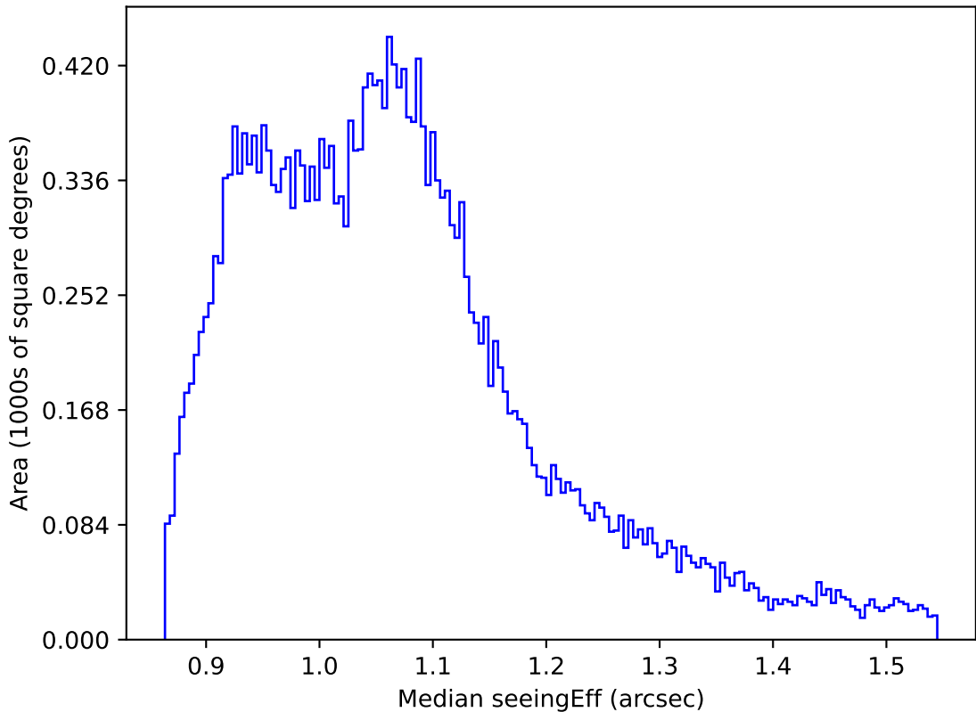
ddf_acor_sf10_lsf20_lsr50_v3.4_10yrs All sky r band: Median seeingEff
