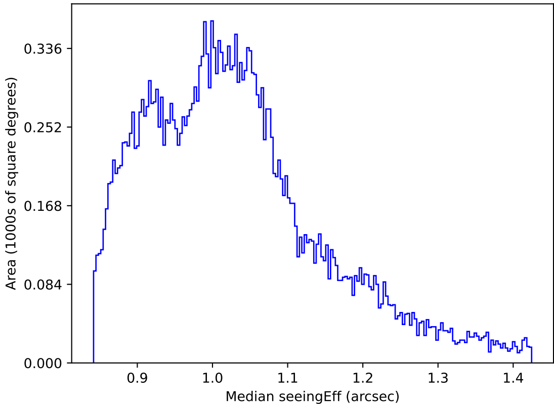
ddf_acor_sf10_lsf20_lsr50_v3.4_10yrs All sky i band: Median seeingEff
