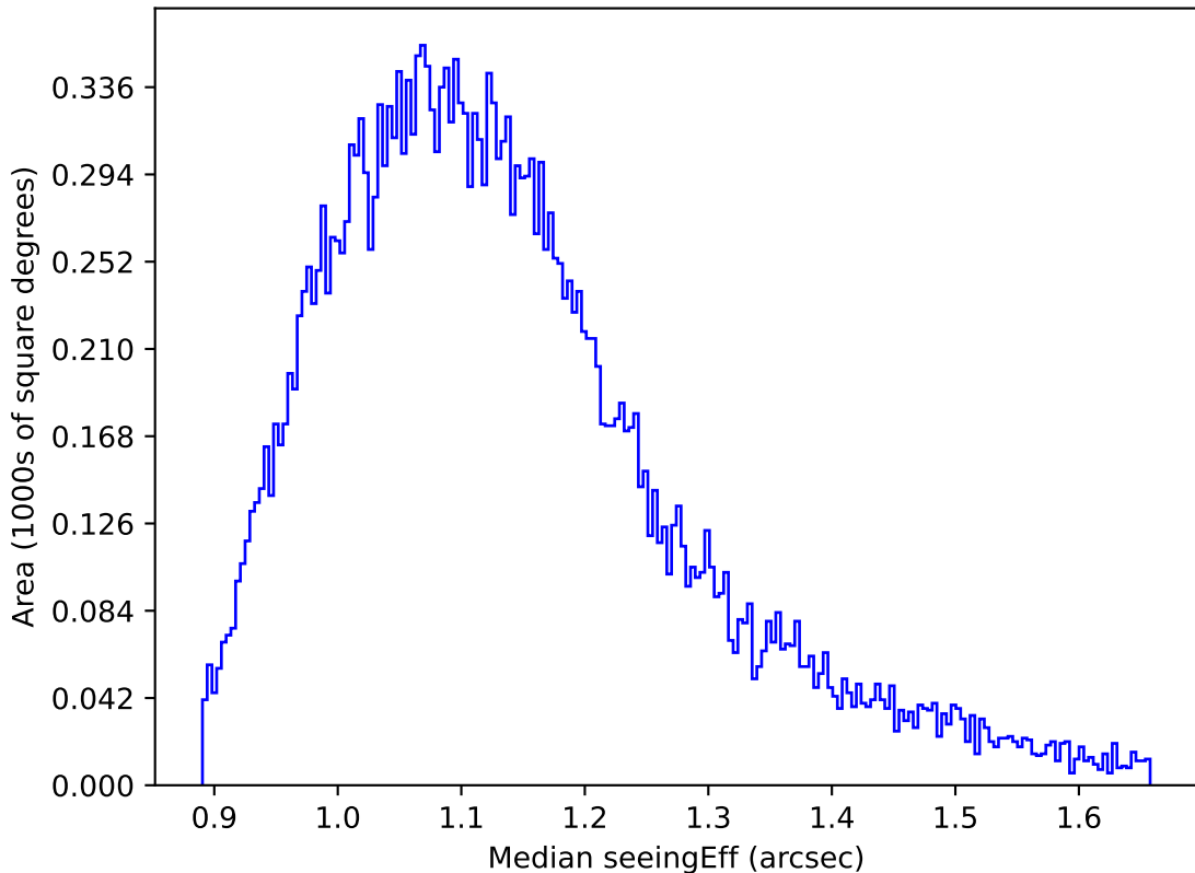
ddf_acor_sf10_lsf20_lsr50_v3.4_10yrs All sky g band: Median seeingEff
