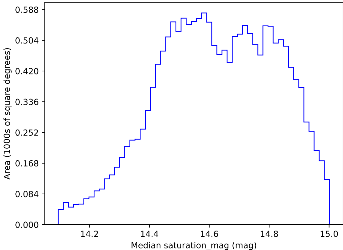
ddf_acor_sf10_lsf20_lsr50_v3.4_10yrs WFD r band: Median saturation_mag
