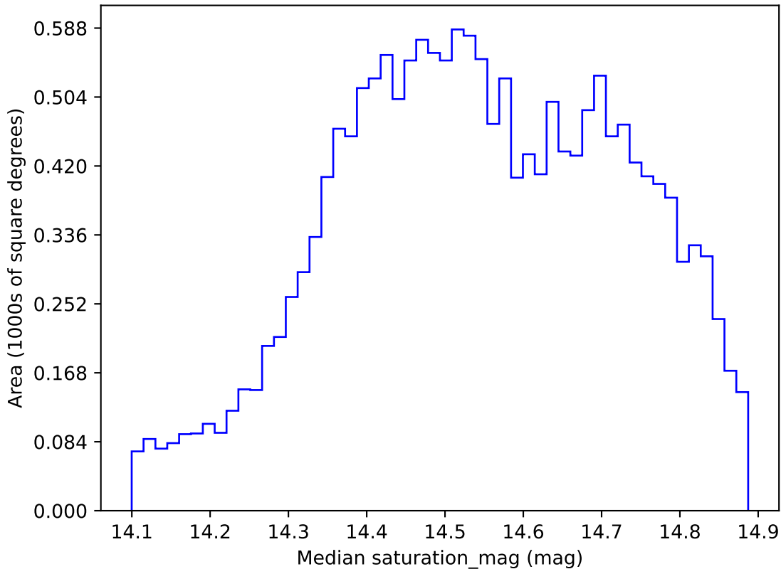
ddf_acor_sf10_lsf20_lsr50_v3.4_10yrs WFD i band: Median saturation_mag
