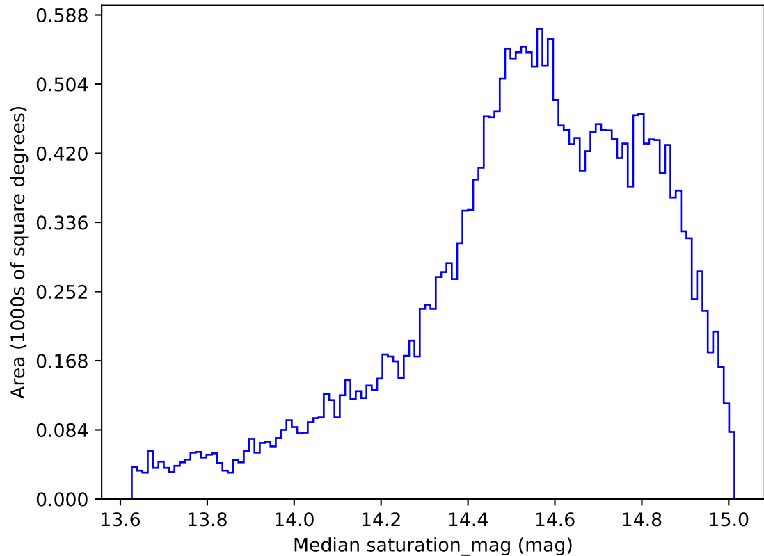
ddf_acor_sf10_lsf20_lsr50_v3.4_10yrs All sky r band: Median saturation_mag
