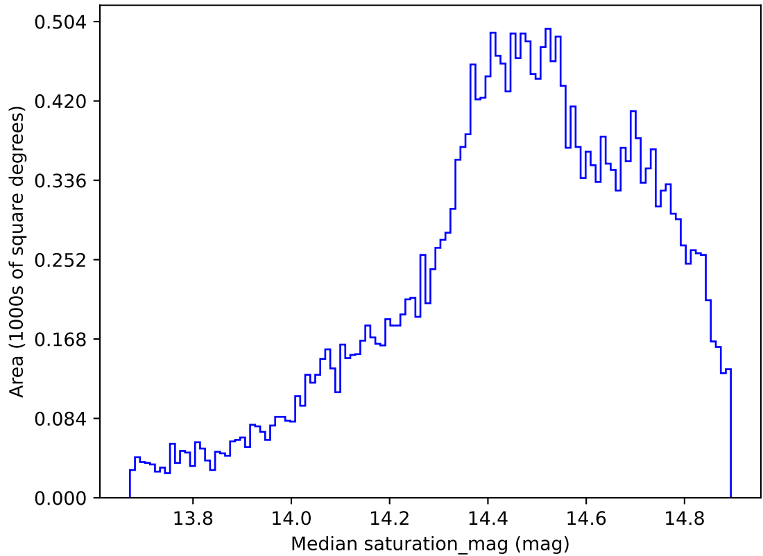
ddf_acor_sf10_lsf20_lsr50_v3.4_10yrs All sky i band: Median saturation_mag
