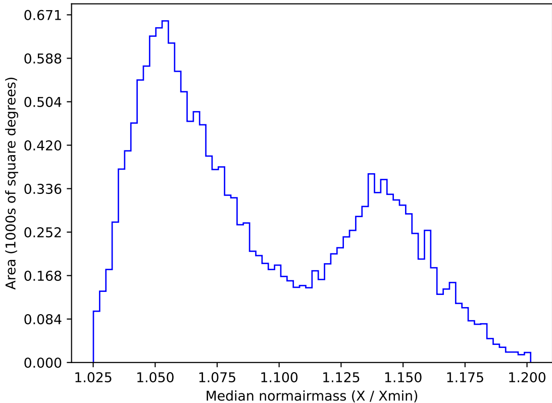
ddf_acor_sf10_lsf20_lsr50_v3.4_10yrs WFD y band: Median normairmass
