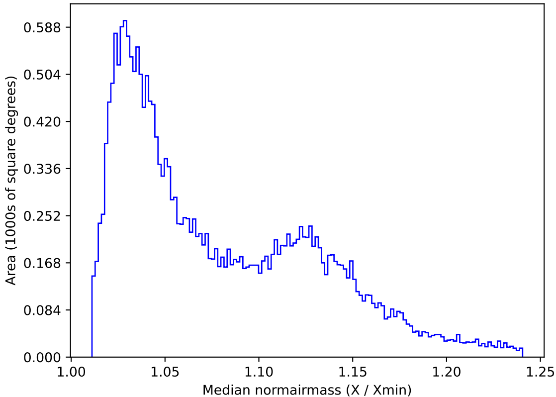
ddf_acor_sf10_ls20_lsr50_v3.4_10yrs All sky u band: Median normairmass
