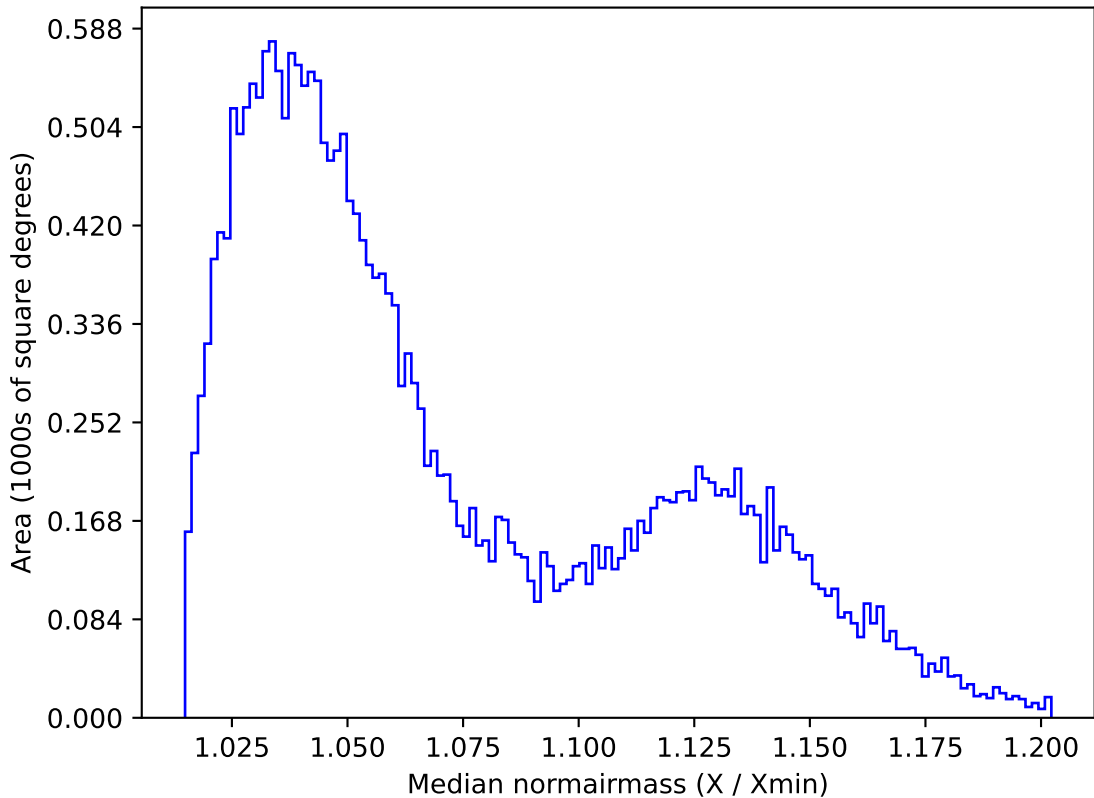
ddf_acor_sf10_lsf20_lsr50_v3.4_10yrs All sky r band: Median normairmass
