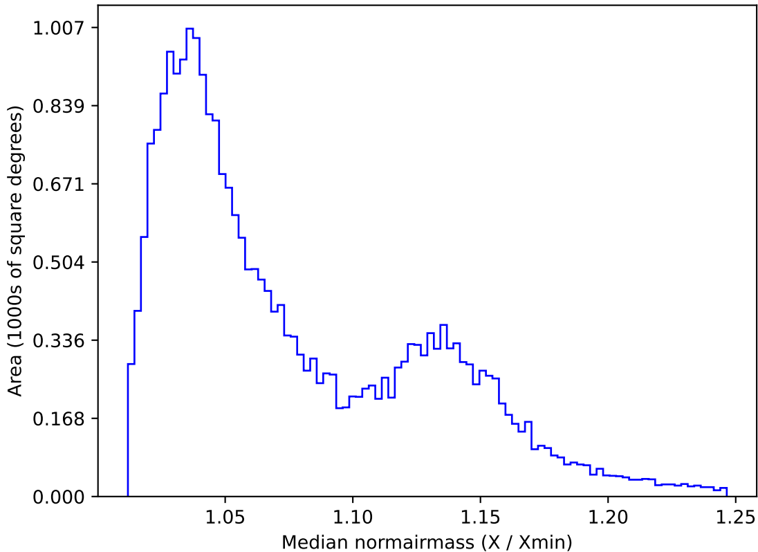
ddf_acor_sf10_lsf20_lsr50_v3.4_10yrs All sky g band: Median normairmass
